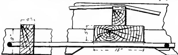
Fig. 1955. Section of Body-bolster and Cross-tie-timber.
